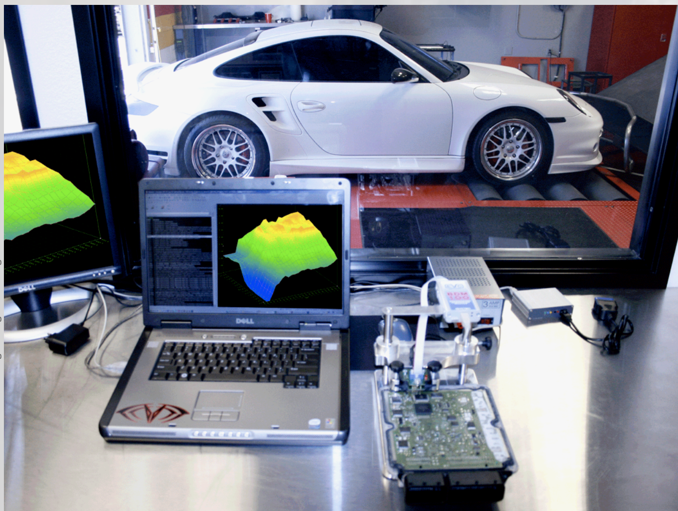
Porsche 997 EVT700 during Intelligent Tuning
